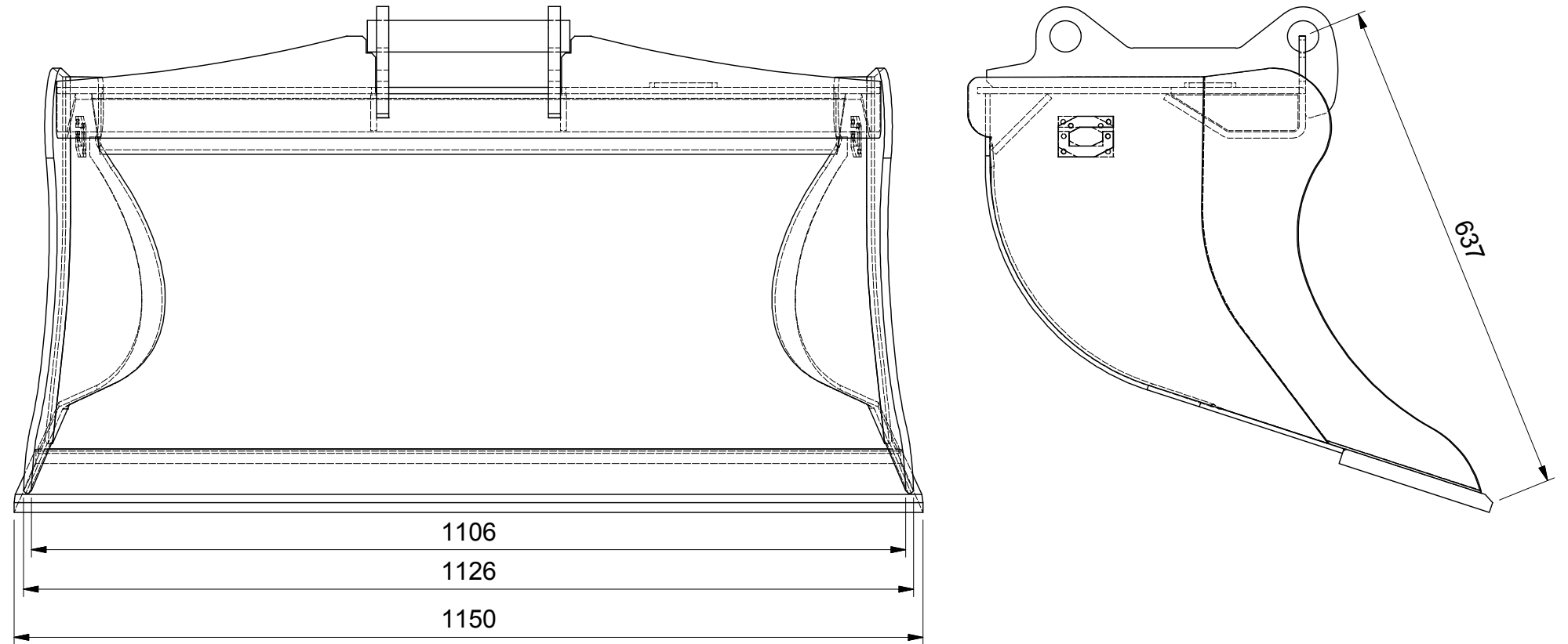
VIEW5 ( 1 : 7.5 )
