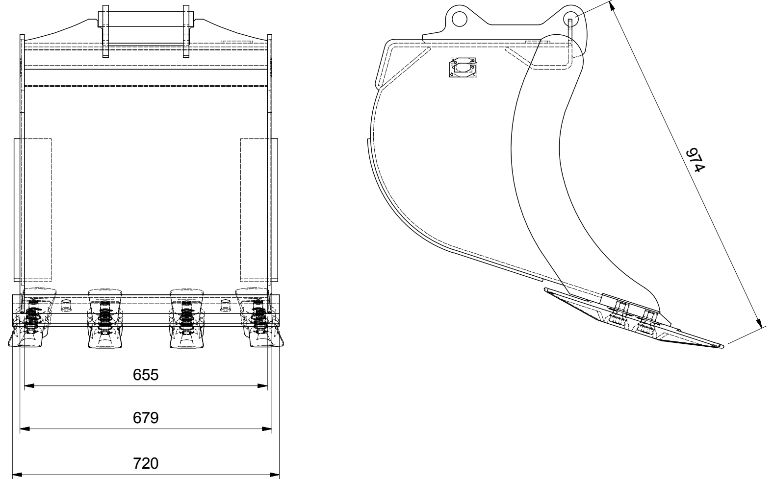
VIEW4 (1 : 10)
