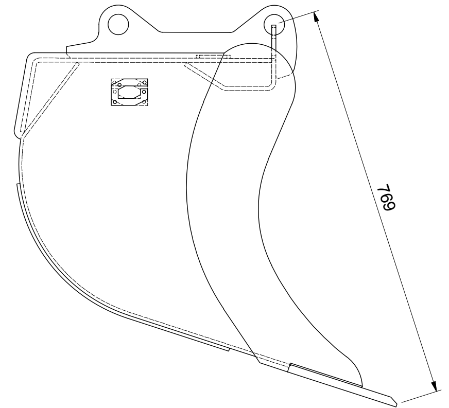
VIEW4 ( 1 : 7.5 )
