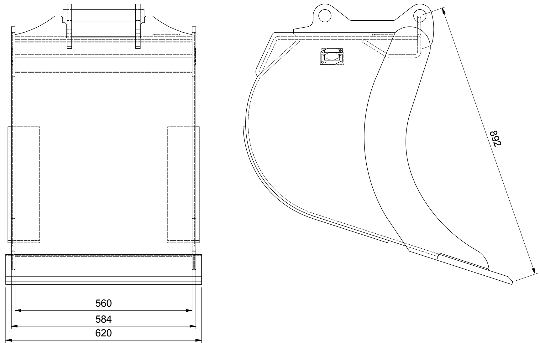
VIEW4 (1:7.5)
