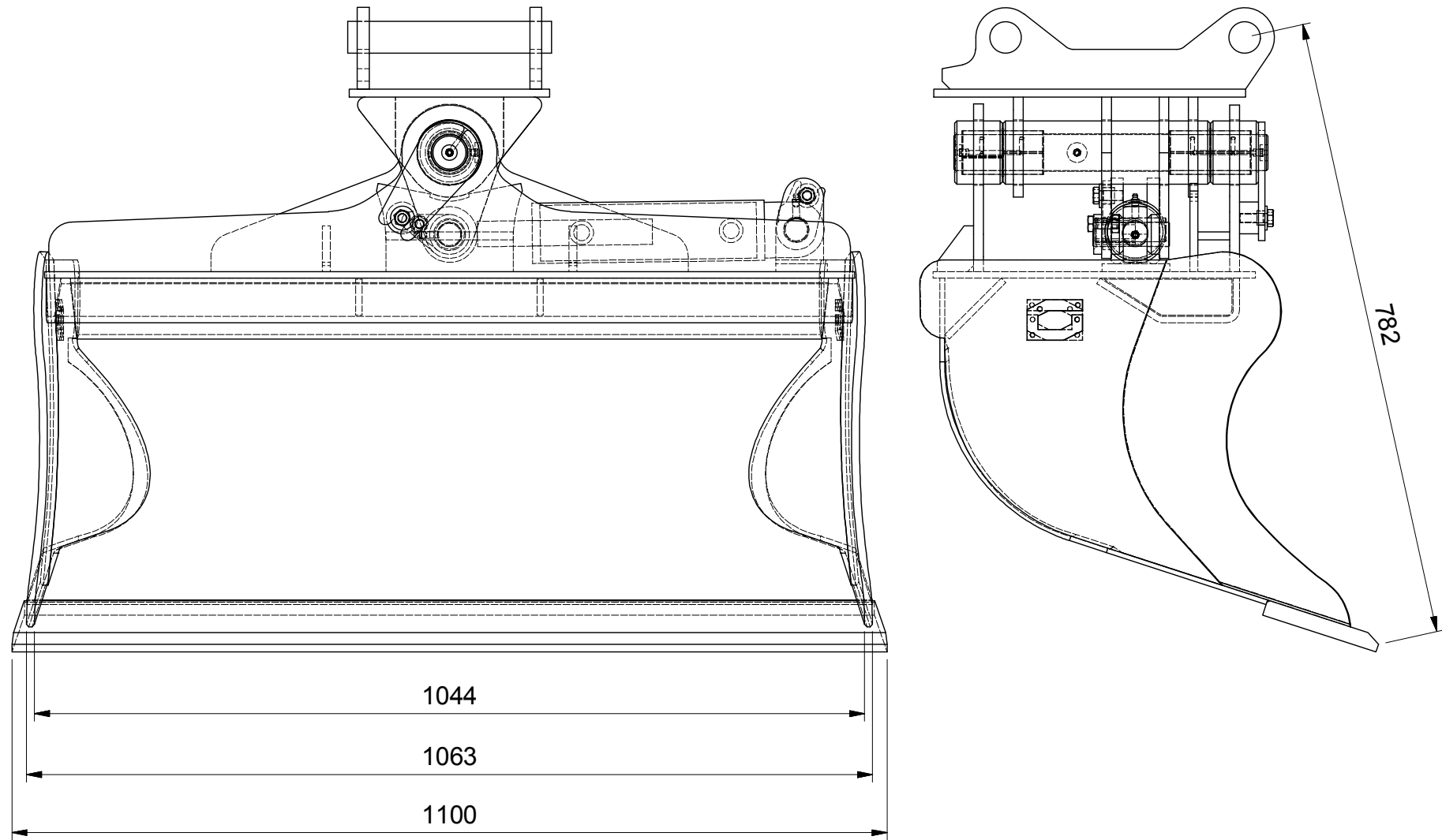
VIEW5 (1 : 7.5)
