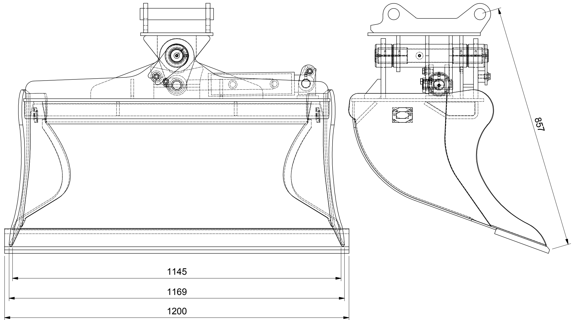
VIEW5 ( 1 : 7.5 )
